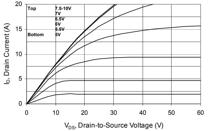
Fig. 4 Extended Typical Output Characteristics
