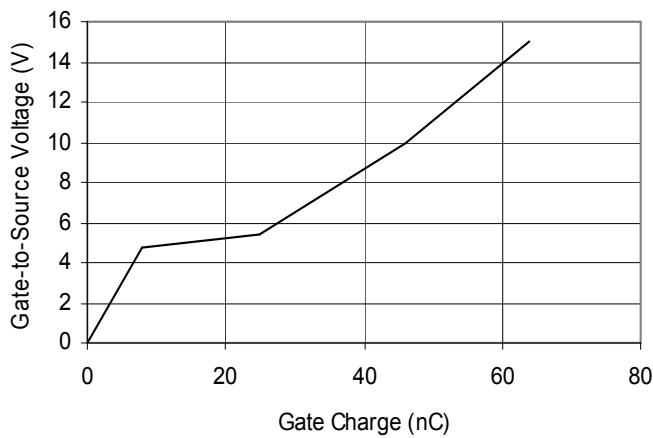
Gate-to-Source Voltage vs. Gate Charge
