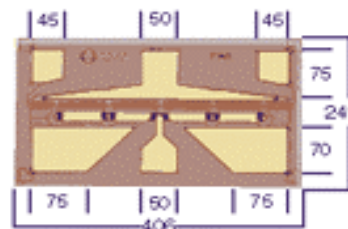
Chip Dimensions: 406 x 241 microns Chip Thickness: 100 microns
