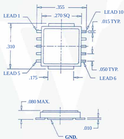
Package 86 (HERMETIC)
