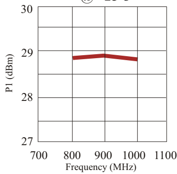
Output Power at P1dB @ +25°C
