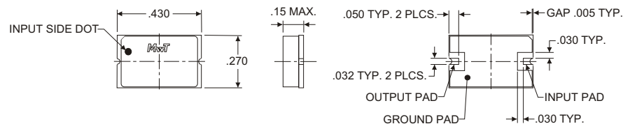
Outline Drawing
