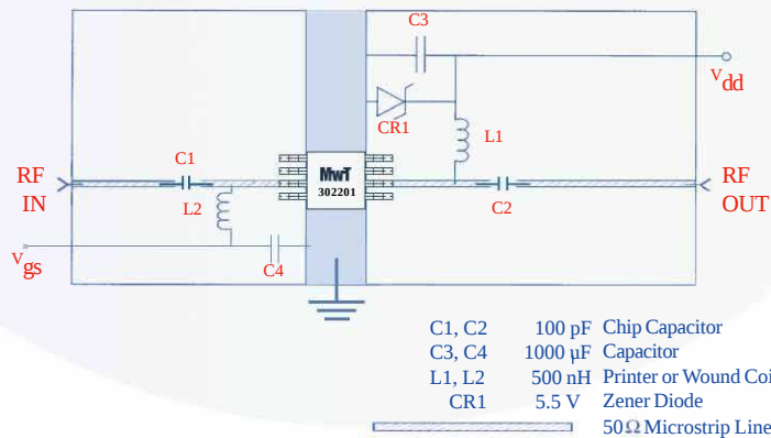
Application Circuit
