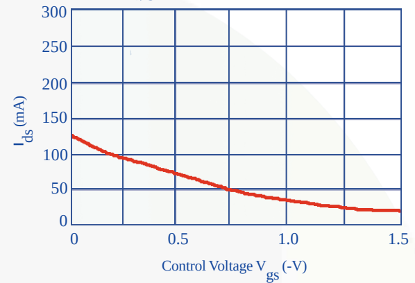
I_{ds} vs. Control Voltage
