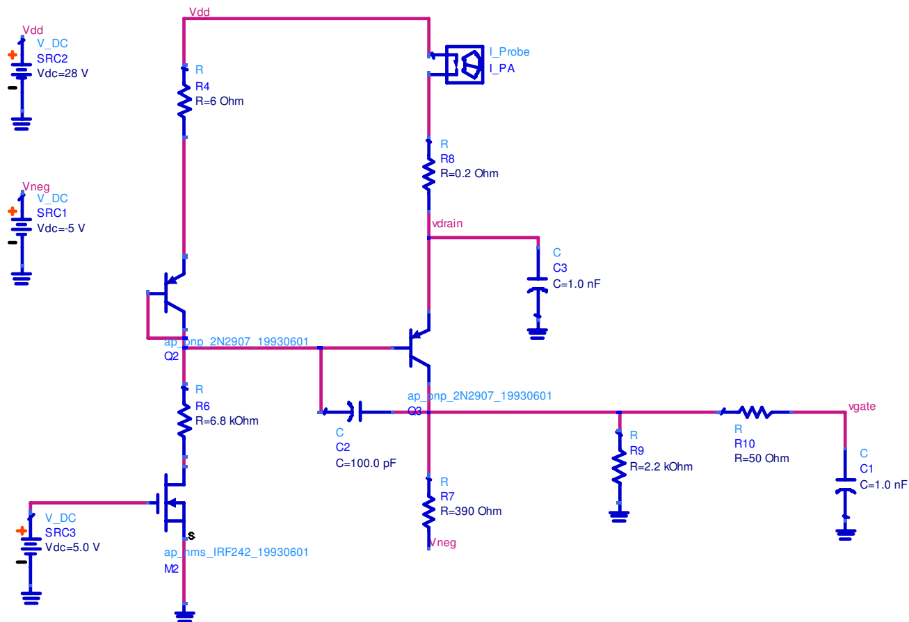
Figure 6 Schematic of Constant Current Loop
