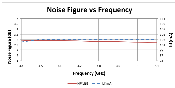
Figure 2 Noise Figure
