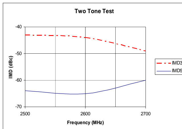
Figure 5 OIP3
