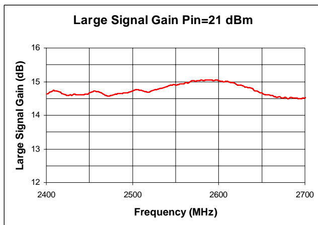
Figure 4 Gain Response
