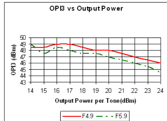
Figure 5 OIP3
