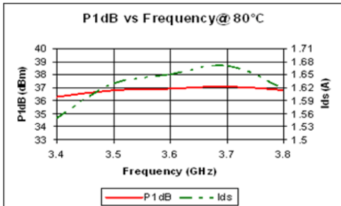
Figure 7 P1dB
