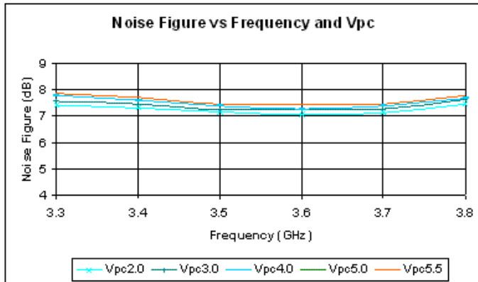
Figure 5 Noise Figure
