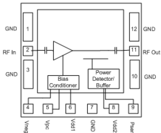
Figure 3 Block Diagram
