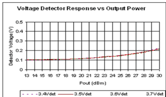
Figure 10 Detector Voltage Response
