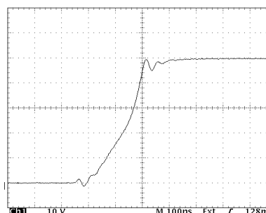
Typical Rise And Settling Times, 50V, 10A, 5 Ohm Load
