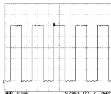
50% Duty Cycle, 250μs Pulse Width, 2KHz Freq. 10A Output
