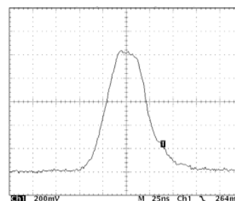
50ns Minimum Pulse Width, <30ns Rise And Fall Times, 10A Output
