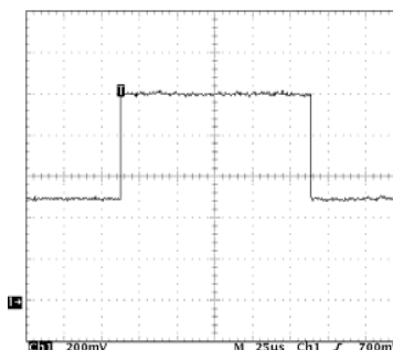
10A, 126μs Pulse On 5A Bias Current (Ground Indicated By "1" Marker)
