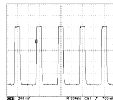
1MHz Frequency (Externally Triggered) 250ns Pulse Width, 10A Output
