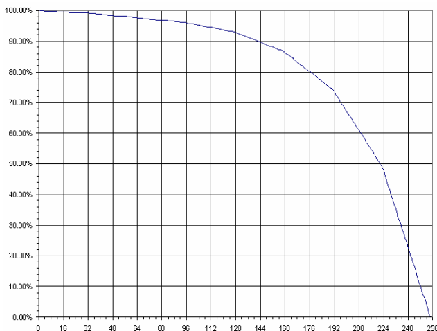
Figure 9: Dynamic Mode Dimming in Logarithmic Mode in percent vs. register 05h, 06h and 07h (0% dimming = full LED brightness)
