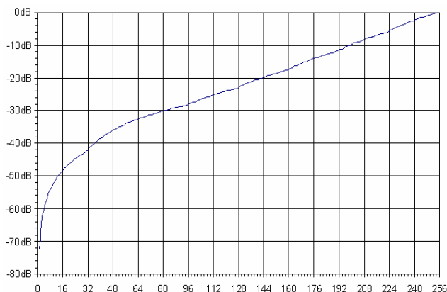
Figure 8: Dynamic Mode Dimming in Logarithmic Mode in dB vs. register 05h, 06h and 07h data (0dB dimming = full LED brightness)
