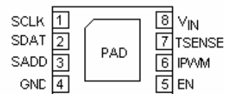
Top View : DFN 8-Lead 3 x 2 mm 2
