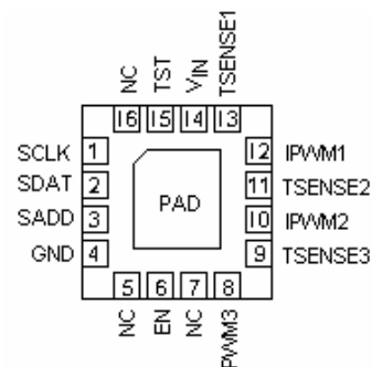
Top View : TQFN 16-Lead 3 x 3 mm 2
