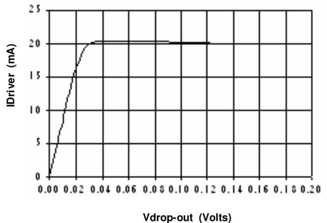
Figure 17 Output Driver Current vs. V_{Drop-Out} Voltage
