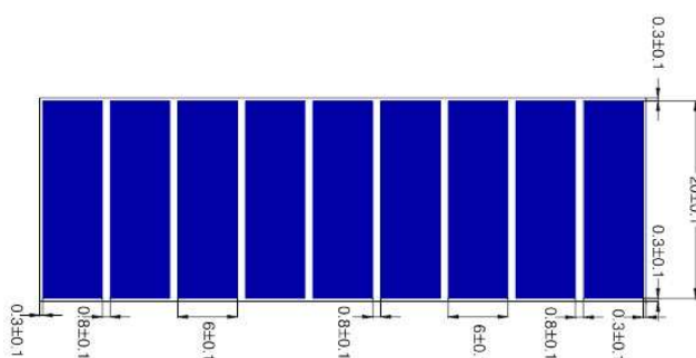
Front-side View
