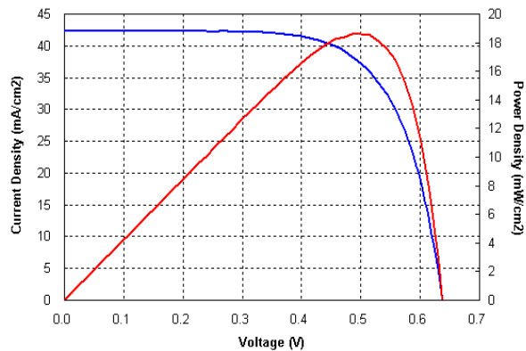
Current-Voltage Characteristics
