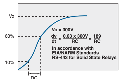
dV/dt Method
