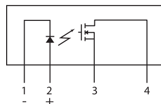
CPC1726 Pinout
