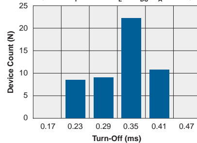
Typical Turn-Off Time ( N=50 , I_F=20\text{mA} , I_L=1\text{A}_{DC} , T_A=25^\circ\text{C} )
