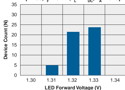
Typical LED Forward Voltage Drop ( N=50 , I_F=10\text{mA} , I_L=1\text{A}_{DC} , T_A=25^\circ\text{C} )
