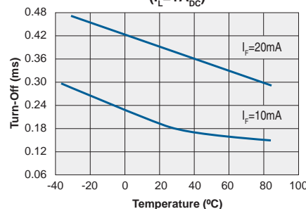
Typical Turn-Off vs. Temperature ( I_L=1\text{A}_{DC} )
