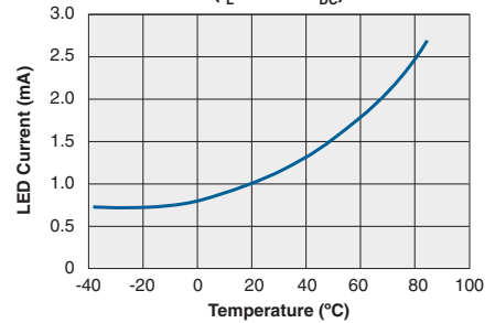
Typical I_F for Switch Dropout vs. Temperature ( I_L=120\text{mA}_{DC} )
