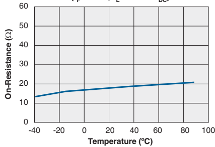
Typical On-Resistance vs. Temperature ( I_F=5\text{mA} , I_L=120\text{mA}_{DC} )
