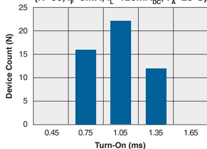
Form-A Typical Turn-On Time (N=50, I_F=5\text{mA} , I_L=120\text{mA}_{\text{DC}} , T_A=25^\circ\text{C} )
