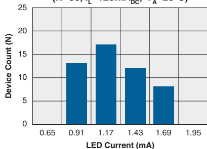
Form-A Typical I_F for Switch Operation (N=50, I_L=120\text{mA}_{\text{DC}} , T_A=25^\circ\text{C} )
