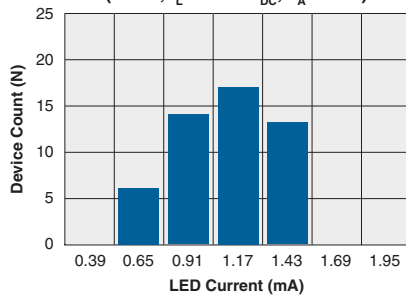
Form-A Typical I_F for Switch Dropout (N=50, I_L=120\text{mA}_{\text{DC}} , T_A=25^\circ\text{C} )
