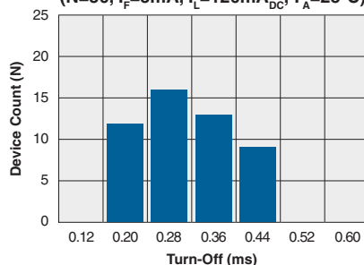
Form-A Typical Turn-Off Time (N=50, I_F=5\text{mA} , I_L=120\text{mA}_{\text{DC}} , T_A=25^\circ\text{C} )
