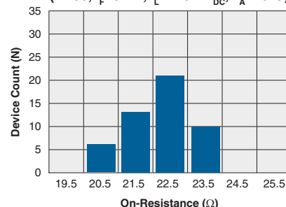
Form-A Typical On-Resistance Distribution (N=50, I_F=5\text{mA} , I_L=120\text{mA}_{\text{DC}} , T_A=25^\circ\text{C} )
