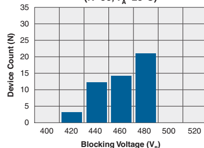
Form-A Typical Blocking Voltage Distribution (N=50, T_A=25^\circ\text{C} )
