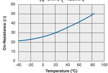
Typical On-Resistance vs. Temperature ( I_F=0\text{mA} , I_L=120\text{mA} )
