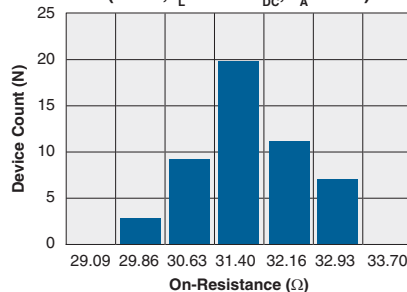
Typical On-Resistance Distribution (N=50, I_L=100\text{mA}_{DC} , T_A=25^\circ\text{C} )
