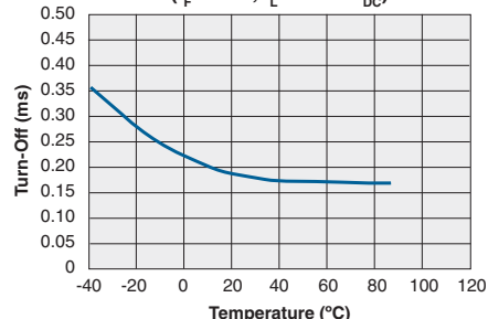
Typical Turn-Off vs. Temperature ( I_F=5\text{mA} , I_L=120\text{mA}_{DC} )
