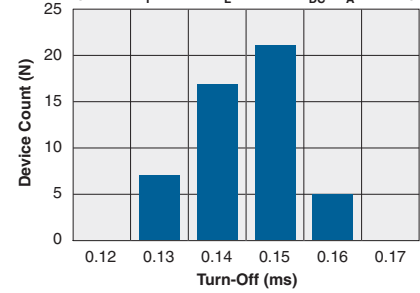
Typical Turn-Off Time (N=50, I_F=5\text{mA} , I_L=200\text{mA}_{DC} , T_A=25^\circ\text{C} )
