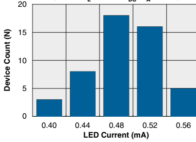
Typical I_F for Switch Dropout (N=50, I_L=200\text{mA}_{DC} , T_A=25^\circ\text{C} )
