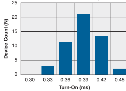
Typical Turn-On Time (N=50, I_F=5\text{mA} , I_L=200\text{mA}_{DC} , T_A=25^\circ\text{C} )
