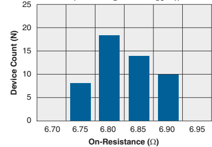
Typical On-Resistance Distribution (N=50, I_F=5\text{mA} , I_L=200\text{mA}_{DC} , T_A=25^\circ\text{C} )
