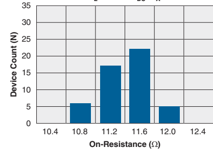
Typical On-Resistance Distribution (N=50, I_L=170\text{mA}_{DC} , T_A=25^\circ\text{C} )
