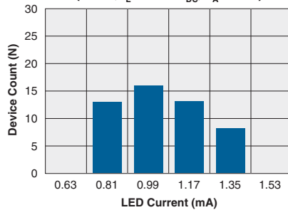
Typical I_F for Switch Operation (N=50, I_L=170\text{mA}_{DC} , T_A=25^\circ\text{C} )
