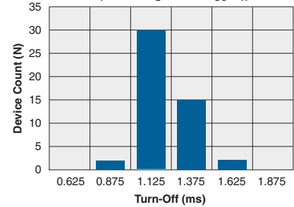
Typical Turn-Off Time (N=50, I_F=5\text{mA} , I_L=170\text{mA}_{DC} , T_A=25^\circ\text{C} )
