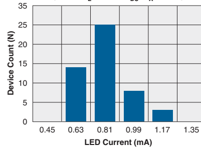
Typical I_F for Switch Dropout (N=50, I_L=170\text{mA}_{DC} , T_A=25^\circ\text{C} )
