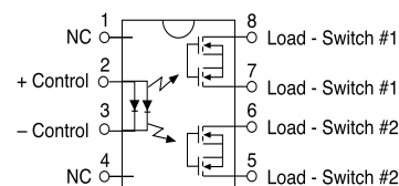
LCA220 Pinout
