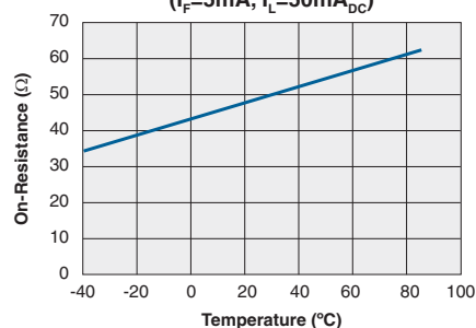
Typical On-Resistance vs. Temperature ( I_F=5\text{mA} , I_L=50\text{mA}_{\text{DC}} )
