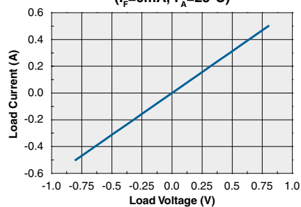
Typical Load Voltage vs. Load Current ( I_F=0\text{mA} , T_A=25^\circ\text{C} )
