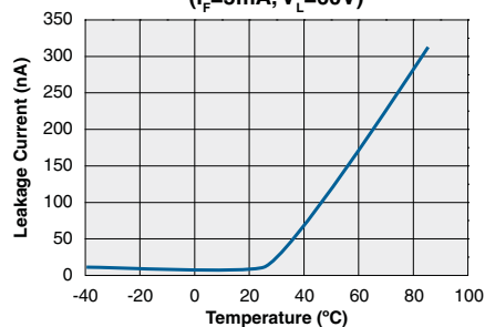
Typical Leakage vs. Temperature Measured Across Pins 4&6 ( I_F=5\text{mA} , V_L=60\text{V} )
