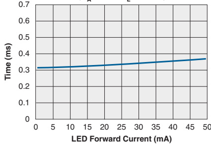
Typical Turn-On vs. LED Forward Current ( T_A=25^\circ\text{C} , I_L=50\text{mA} )
