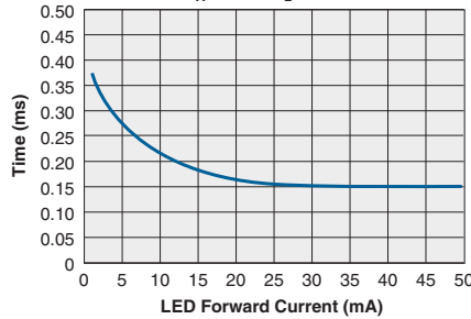
Typical Turn-Off vs. LED Forward Current ( T_A=25^\circ\text{C} , I_L=50\text{mA} )
