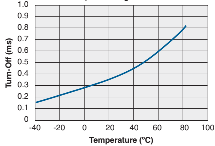
Typical Turn-Off vs. Temperature ( I_F=2\text{mA} , I_L=50\text{mA} )
