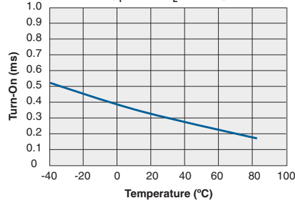
Typical Turn-On vs. Temperature ( I_F=2\text{mA} , I_L=50\text{mA} )
