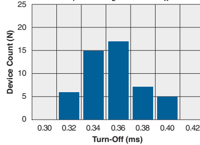
Typical Turn-Off Time (N=50, I_F=2\text{mA} , I_L=150\text{mA} , T_A=25^\circ\text{C} )
