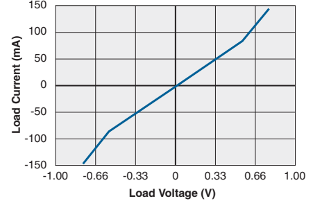
Typical Load Current vs. Load Voltage ( T_A=25^\circ\text{C} )
