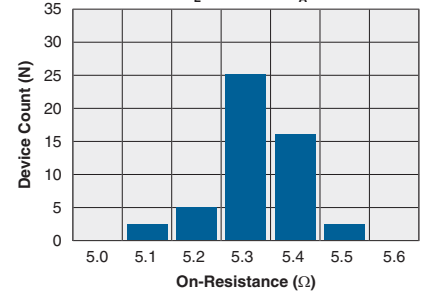
Typical On-Resistance Distribution (N=50, I_L=150\text{mA} , T_A=25^\circ\text{C} )
