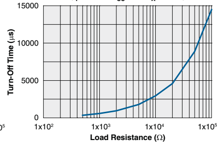
Turn-Off Time vs. Load Resistance ( I_F=1\text{mA} , V_{CC}=5\text{V} , T_A=25^\circ\text{C} )
