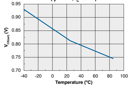
V_{CE(sat)} vs. Temperature ( I_F=1\text{mA} , I_C=3\text{mA} )
