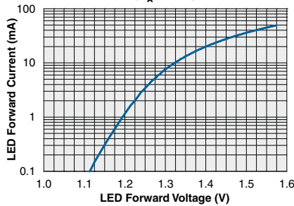
LED Voltage vs. Current (Log) ( T_A=25^\circ\text{C} )
