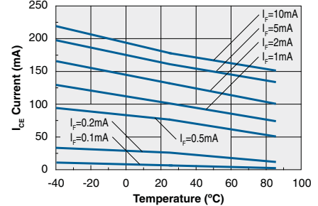
IC Current vs. Temperature ( V_{CE}=5\text{V} )
