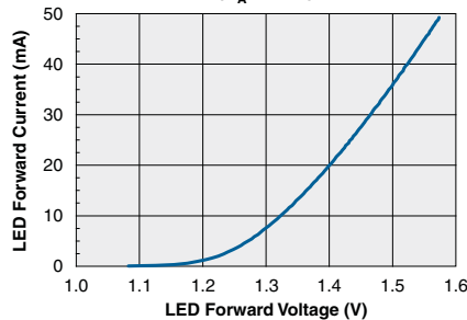
LED Voltage vs. Current ( T_A=25^\circ\text{C} )
