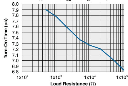
Turn-On Time vs. Load Resistance ( I_F=1\text{mA} , V_{CC}=5\text{V} , T_A=25^\circ\text{C} )
