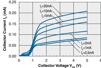
Typical Collector Current vs. Collector Voltage ( T_A=25^\circ\text{C} )
