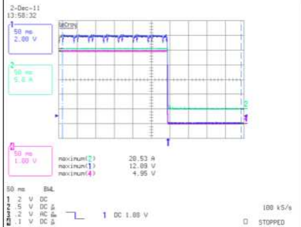
Figure 17: OCP Trigger Timing Ch 1: V_o Ch 2: I_o Ch 4: DC\_OK
