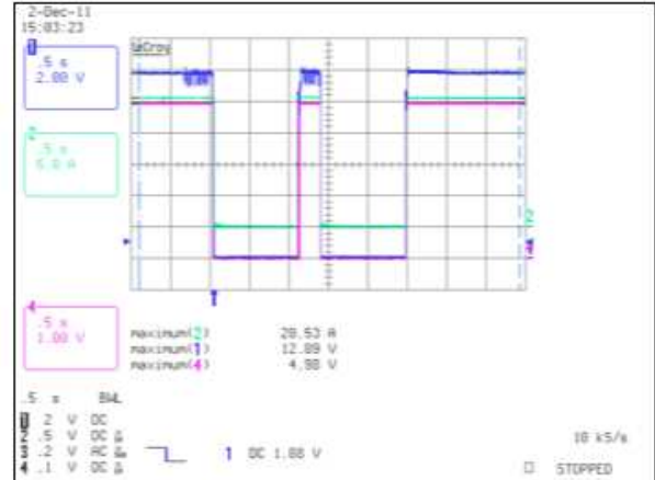
Figure 16: OCP Recovery Timing Ch 1: V_o Ch 2: I_o Ch 4: DC\_OK
