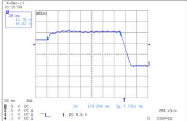
Figure 15: OUTPUT OVP Trigger Timing Full Load: V_o = 16.7A , V_{STD} = 0A
