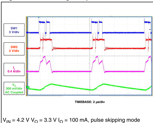
Figure 15. Buck region operation
