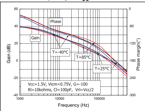
Figure 4. Voltage gain and phase vs. frequency at V_{CC} = 1.5\text{ V}
