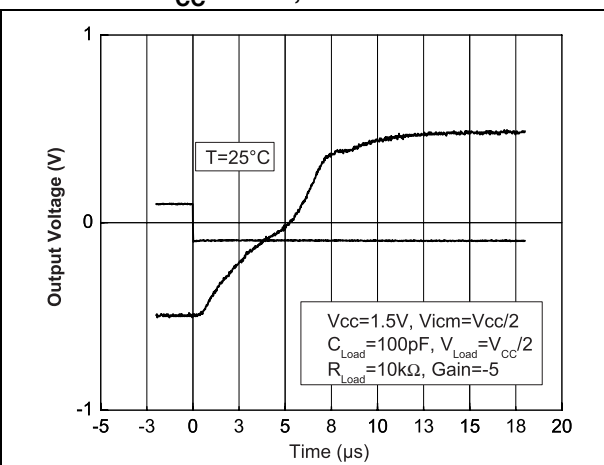
Figure 6. Positive slew rate vs. time at V_{CC} = 1.5\text{ V} ,
