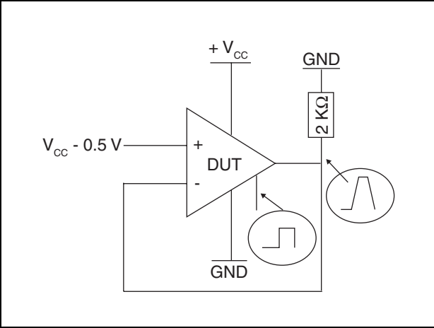
Figure 17. Turn-on time, V_{CC} = 5\text{ V} , Vout pulled down, T = 25^\circ\text{ C}
