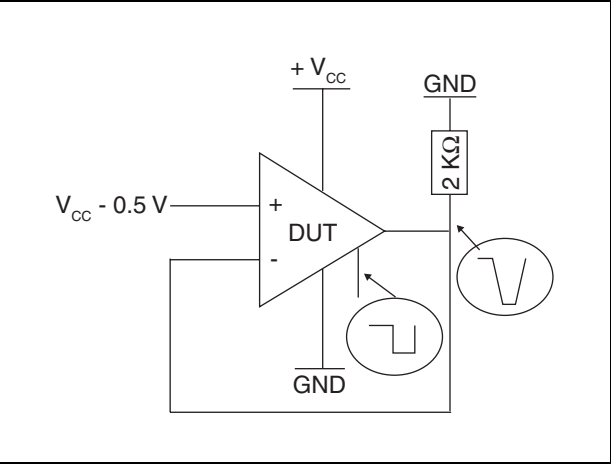
Figure 18. Turn-off time, V_{CC} = 5\text{ V} , Vout pulled down, T = 25^\circ\text{ C}
