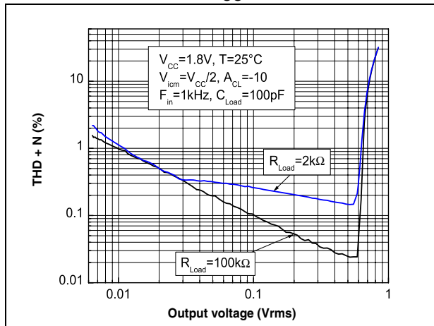
Figure 9. Distortion + noise vs. output voltage at V_{CC} = 1.8\text{ V}
