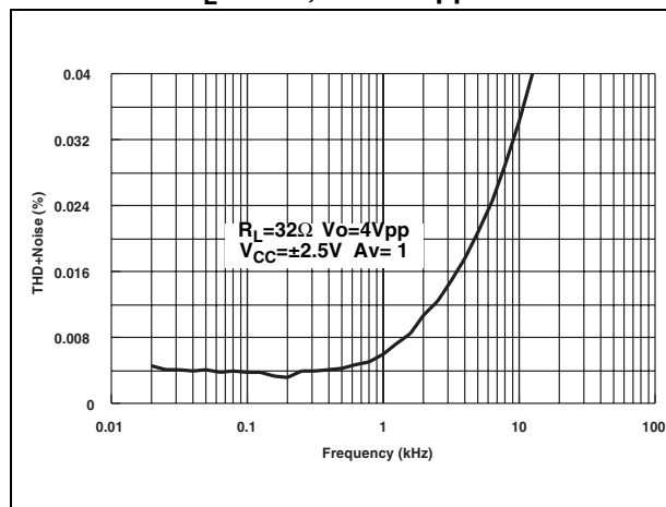
Figure 7. THD + noise vs. frequency, R_L = 32\ \Omega , V_o = 4\ V_{pp}
