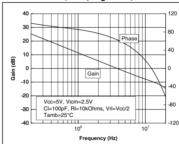
Figure 3. Voltage gain and phase vs. frequency, C_L = 100 \text{ pF}
