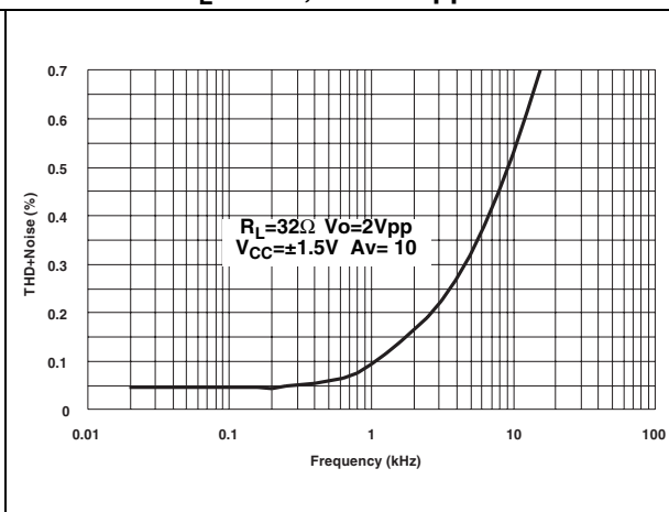
Figure 8. THD + noise vs. frequency, R_L = 32\ \Omega , V_o = 2\ V_{pp}
