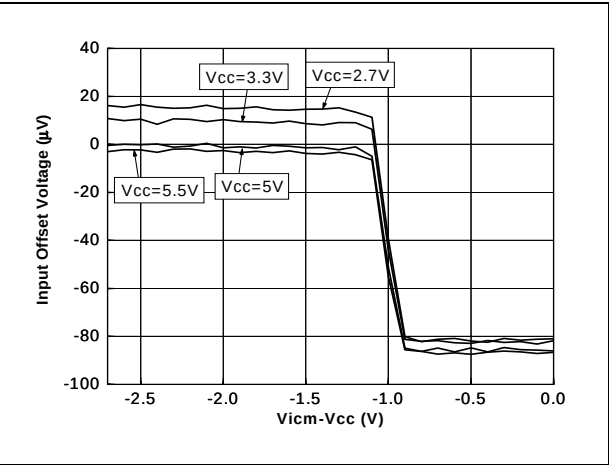
Figure 6. Input offset voltage vs. input common mode voltage at T=25^{\circ}C
