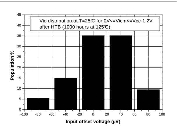
Figure 4. Input offset voltage distribution for V_{icm} \leq V_{CC}-1.2V at T=25^{\circ}C after HTB
