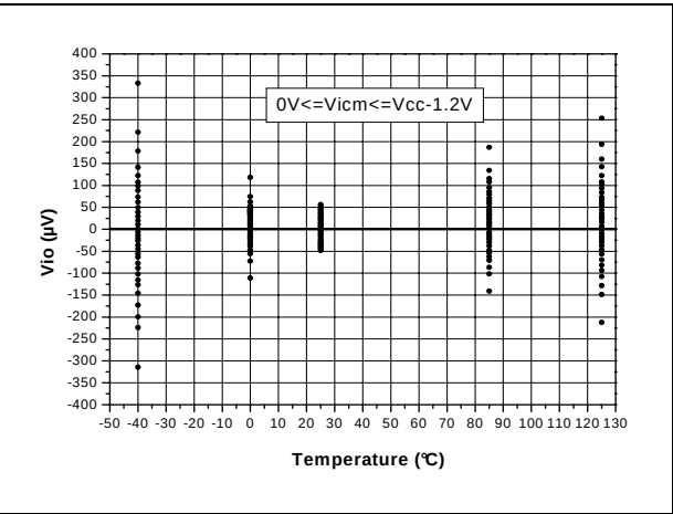
Figure 2. Input offset voltage distribution vs. temperature for V_{icm} \leq V_{CC}-1.2V
