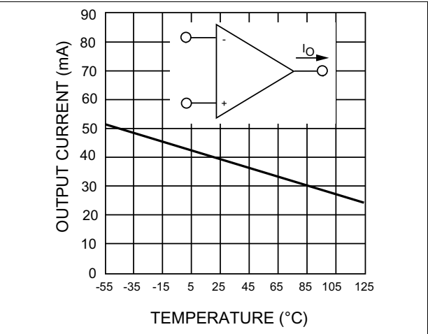
Figure 10. Current limiting
