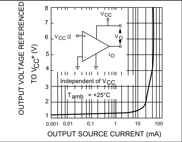
Figure 8. Output characteristics
