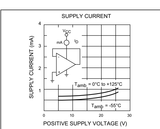
Figure 12. Supply current
