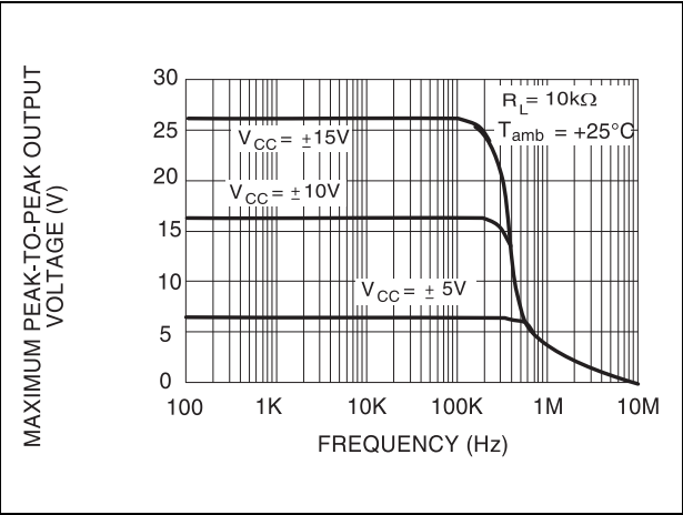
Figure 3. Maximum peak-to-peak output voltage versus frequency ( R_L = 10\text{k}\Omega )
