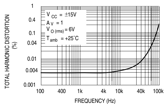
Figure 18. Total harmonic distortion versus frequency
