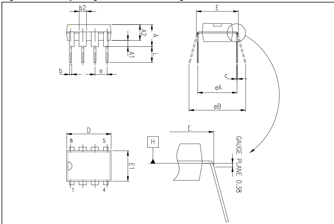
Figure 10. DIP8 package mechanical drawing
