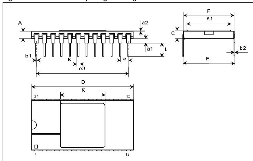
Figure 7. Ceramic DIL-24 package drawings
