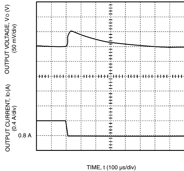
Figure 4. LC016AJ Typical Output Voltage for a Step Load Change from 50% to 25%
