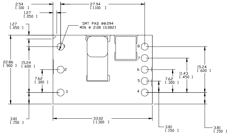
SMT Recommended Pad Layout (Component Side View)
