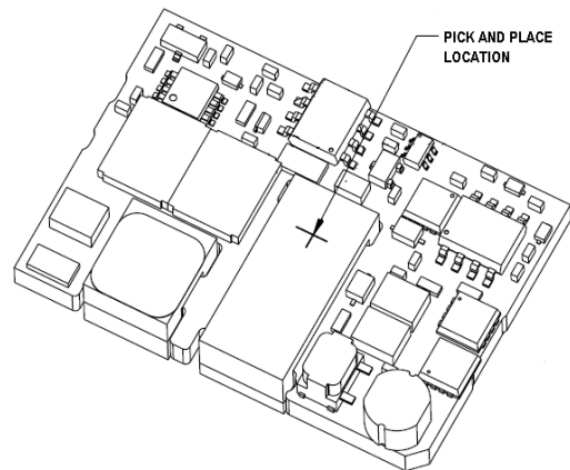
Figure 16. Pick and Place Location.
