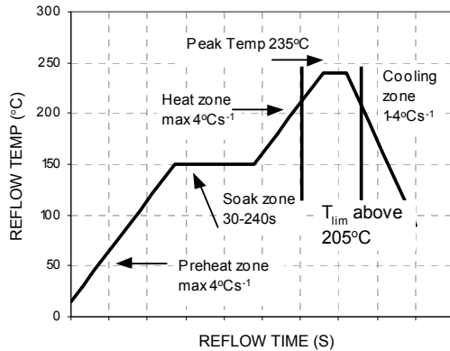
Figure 17. Reflow Profile for Tin/Lead (Sn/Pb) process
