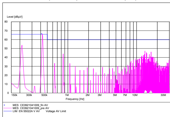
Figure 15. KW015A0F Average Conducted Emissions with EN 55022 Class A limits, no external filter ( V_{IN} = V_{IN,NOM} , I_o = 0.85 I_{o,max} ).
