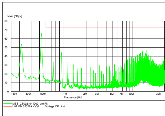
Figure 14. KW015A0F Quasi Peak Conducted Emissions with EN 55022 Class A limits, no external filter ( V_{IN} = V_{IN,NOM} , I_o = 0.85 I_{o,max} )
