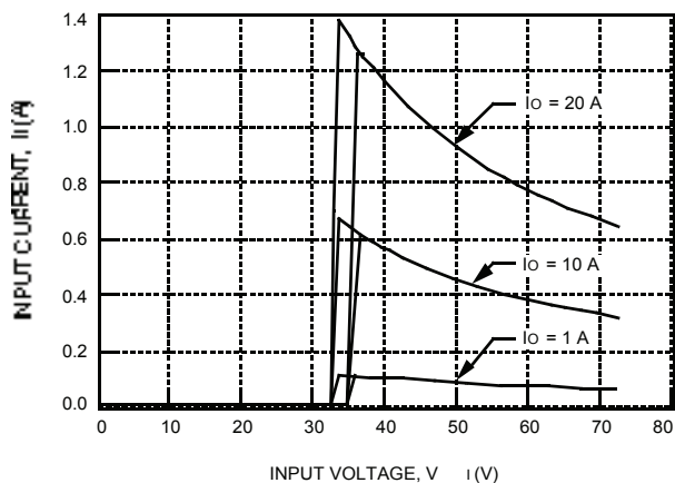
Figure 1. Typical JW100M Input Characteristics at Room Temperature
