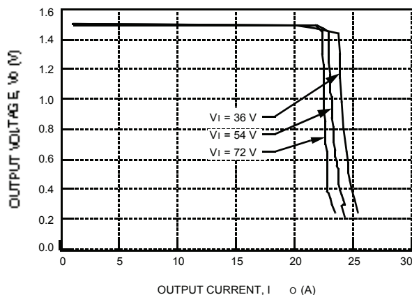
Figure 2. Typical JW100M Output Characteristics at Room Temperature
