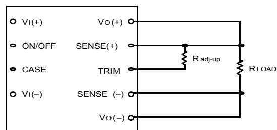
Figure 12. Circuit Configuration to Increase Output Voltage
