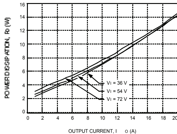
Figure 16. JW100M Power Dissipation vs. Output Current at 25 °C
