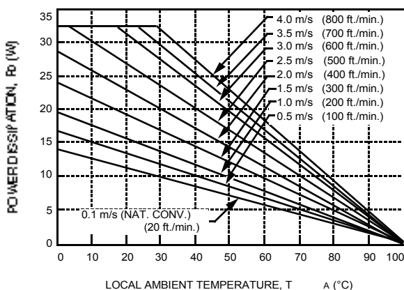
Figure 15. Forced Convection Power Derating with No Heat Sink; Either Orientation
