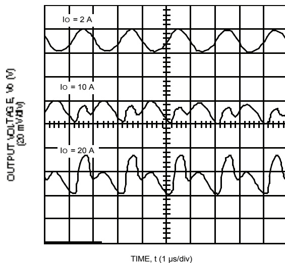
Figure 4. Typical JW100M Output Ripple Voltage at Room Temperature, 48 V Input
