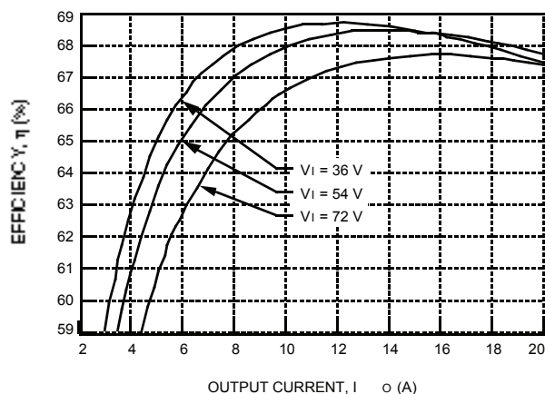
Figure 3. Typical JW100M Converter Efficiency vs. Output Current at Room Temperature
