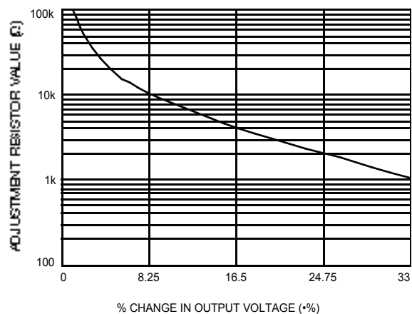
Figure 11. Resistor Selection for Decreased Output Voltage
