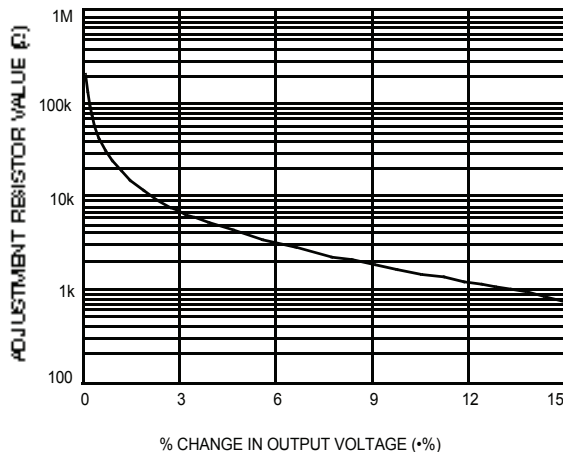
Figure 13. Resistor Selection for Increased Output Voltage
