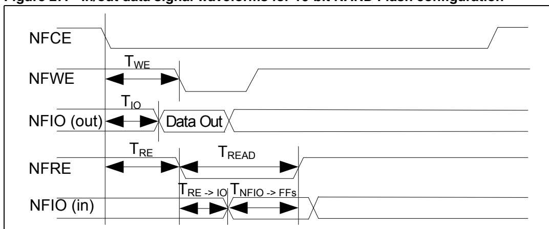
Figure 27. In/out data signal waveforms for 16-bit NAND Flash configuration
