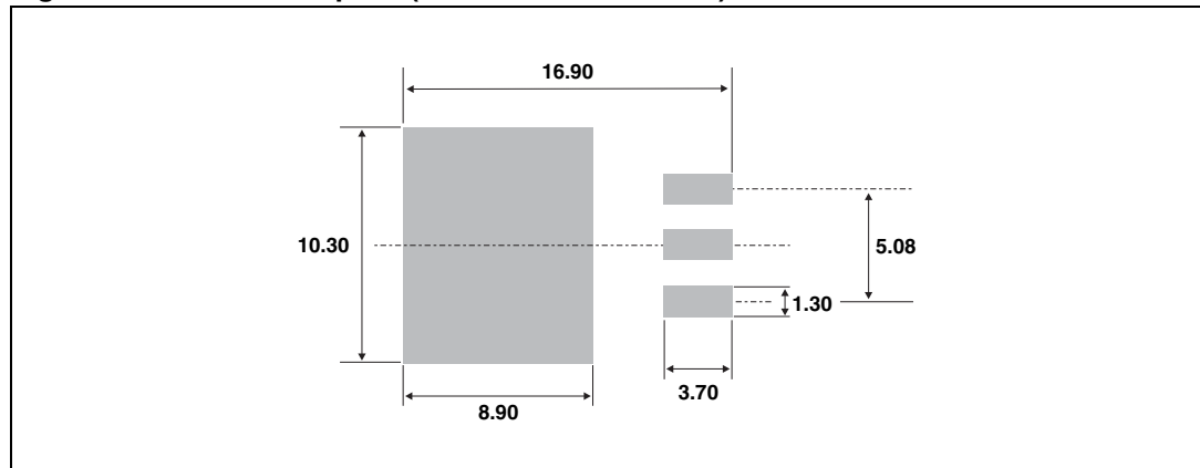
Figure 12. D 2 PAK footprint (all dimensions in mm)
