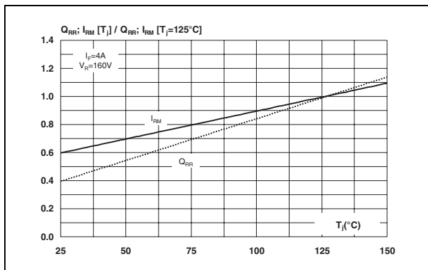
Figure 13. Dynamic parameters versus junction temperature
