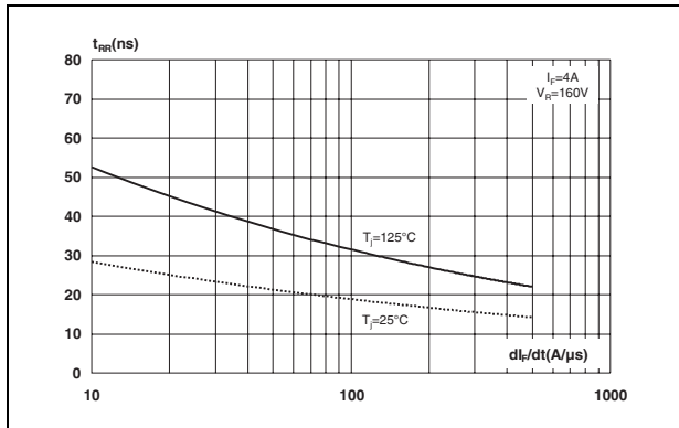
Figure 11. Reverse recovery time versus di_F/dt (typical values)
